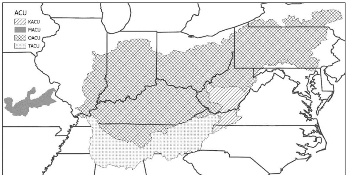
Figure 1. Eastern hellbender adaptive capacity units (ACUs). KACU=Kanawha River drainage; MACU=Missouri; OACU=Ohio River-Susquehanna River drainages; TACU=Tennessee River drainage.
